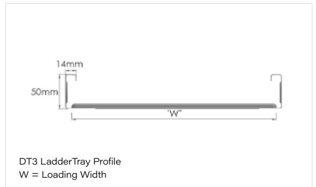
DT3 LadderTray
